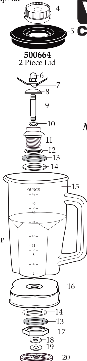
501427 Container with Blending Assembly
